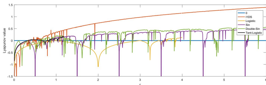
Fig. 1 Lyapunov exponent for different chaotic maps [33]
